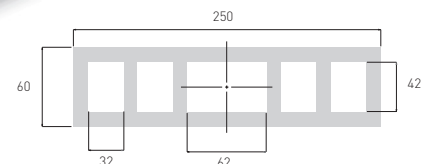
B-250x60
