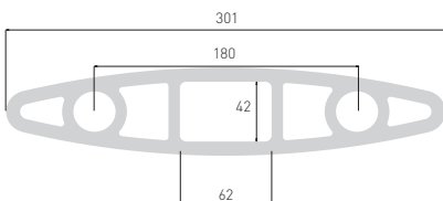
BO-300x62
