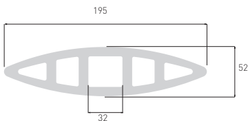
BO-200x50
