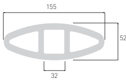
BO-160x50
