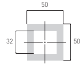
B-5x5 curvo
